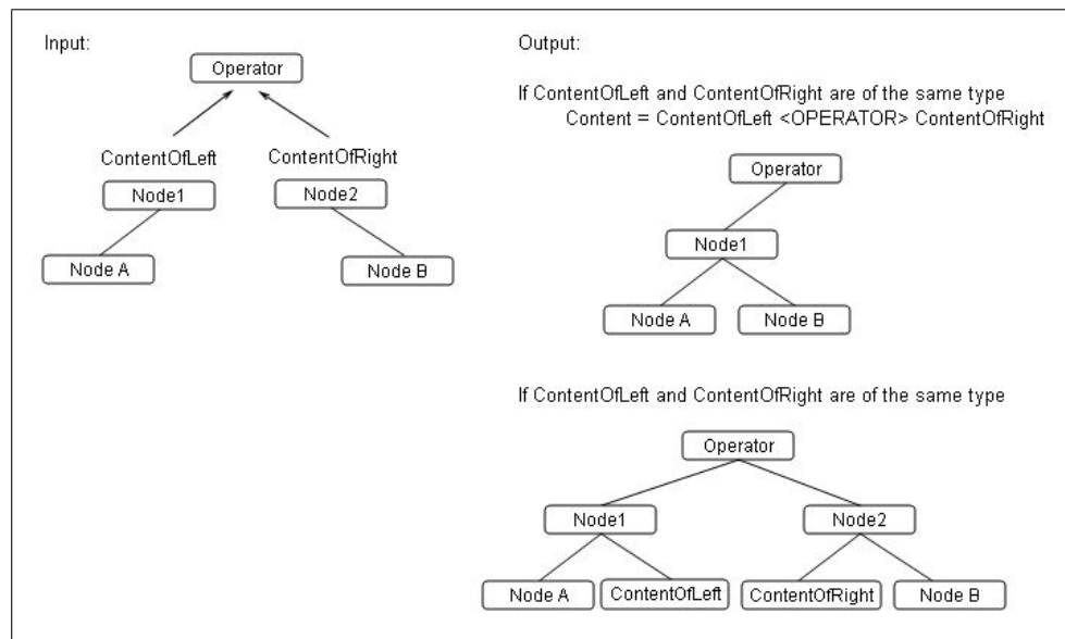
Figure C.5: Content and node coming from both children
