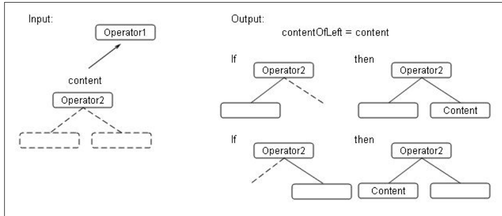
Figure C.1: Content and node (same with the current operator) coming from left child (opposite child result order for input yields opposite output)
