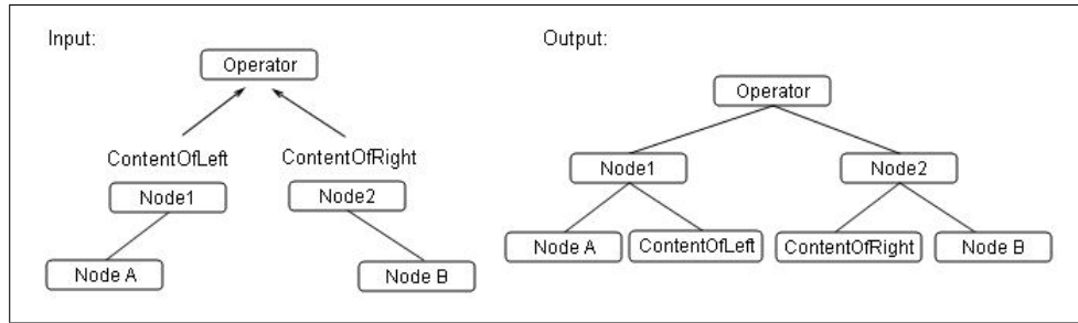
Figure C.3: Content and node coming from both children
