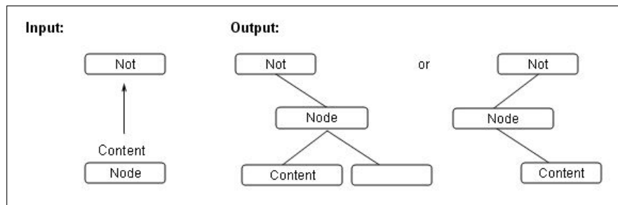
Figure E.2: Content and node coming from child
