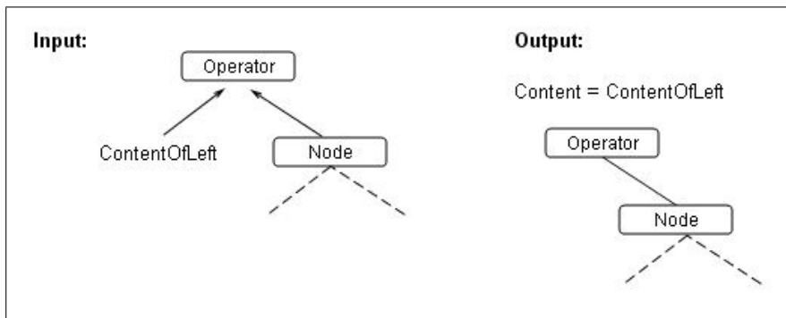
Figure B.11: Content from left child and node coming from right child (opposite input yields opposite output)
