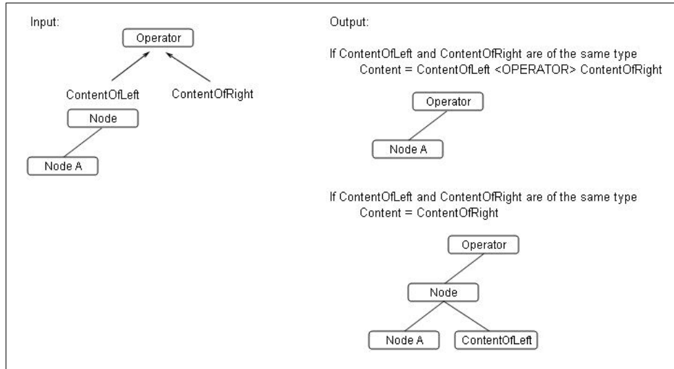
Figure C.4: Content and node coming from left child and content coming from right child (opposite child result order for input yields opposite output)
