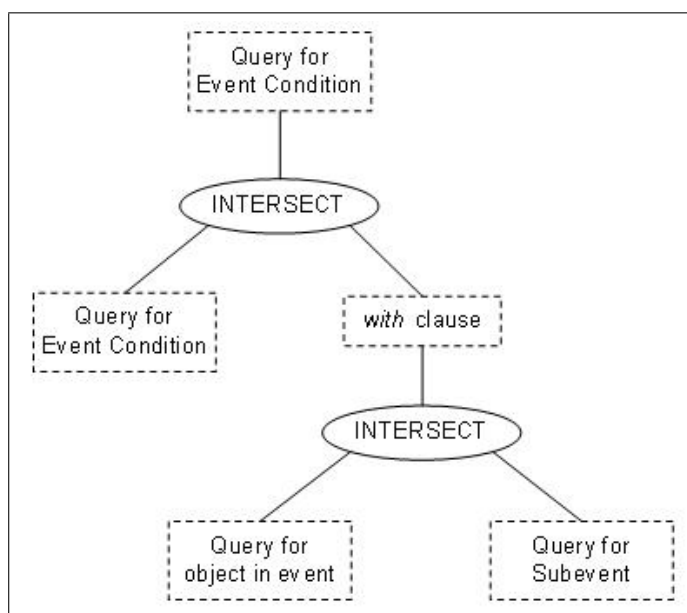
Figure 5.3: The subtree for the event condition of the sample query (rectangular nodes represent subparse tree equivalents of the corresponding condition types)
