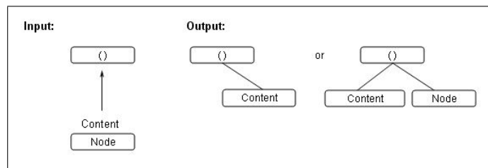
Figure D.2: Content and node coming from child
