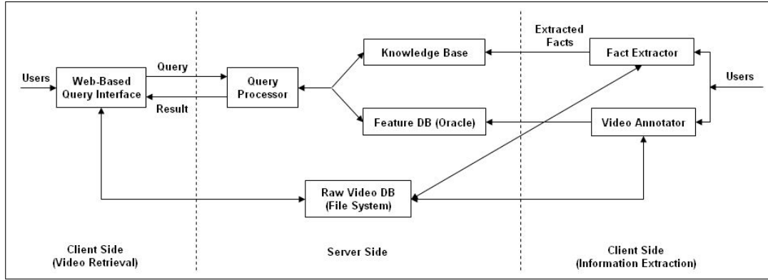
Figure 3.1: BilVideo System Architecture
