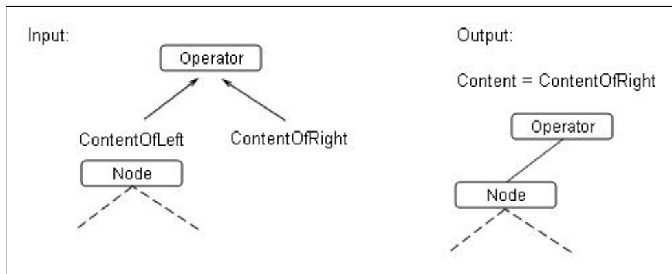
Figure C.2: Content and node coming from left child and content coming from right child (opposite child result order for input yields opposite output)
