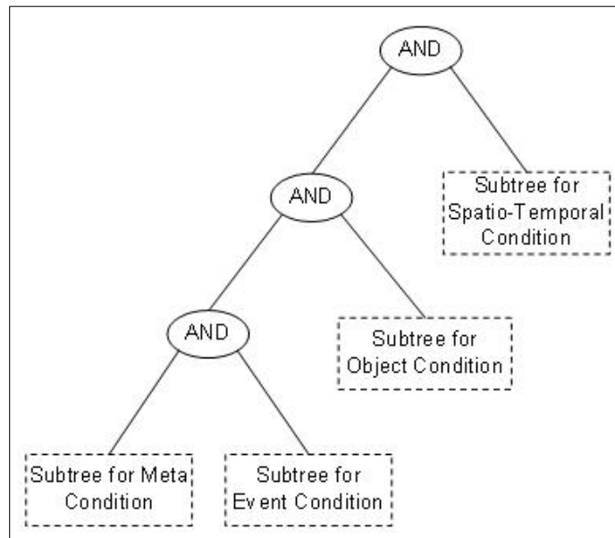
Figure 5.2: The parse tree for the conditions in the where clause of the sample query (rectangular nodes represent subparse tree equivalents of the corresponding condition types)
