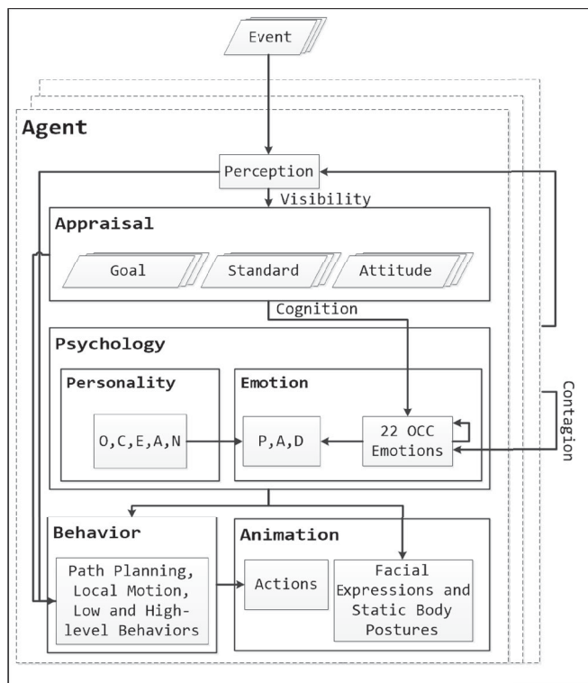
Fig. 2. The components that make up an agent.
