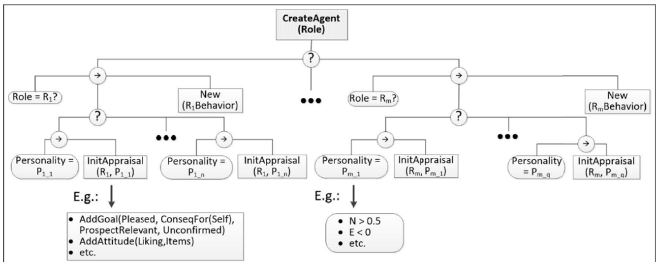
Fig. 6. Behavior tree for initializing an agent in a crowd.
