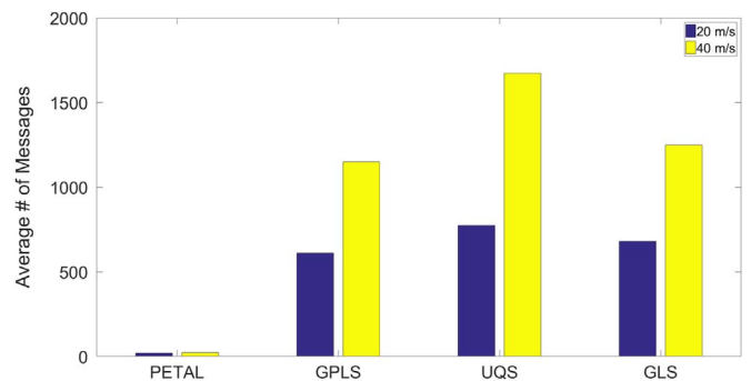
Fig. 15. Average number of location update messages sent per node for different speeds of swarm movement (2500 m×2500 m field, random waypoint mobility, transmission range=250 m, time=500 units).
