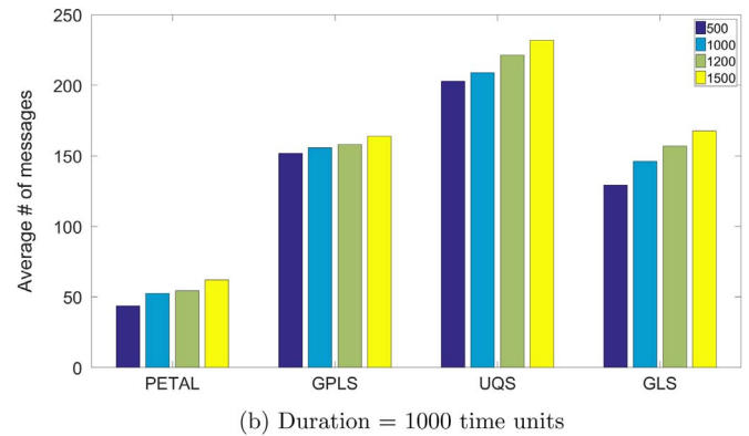
Fig. 7. Average number of location update messages sent per node for different number of nodes (2500 m×2500 m field, random waypoint mobility, transmission range=250 m).
