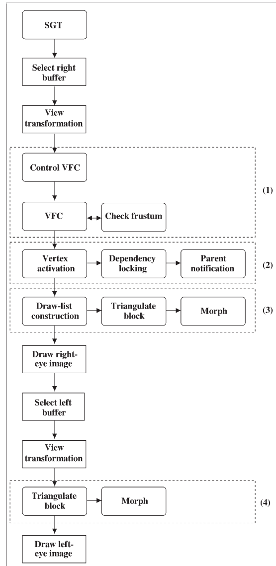
Fig. 8. The process flow diagram of the proposed framework for stereoscopic visualization. This diagram shows the invocation order of the presented algorithms. The data worked on by the processes in the dashed blocks are 1) the whole quad-tree, 2) the view-frustum culled data, 3) the activated blocks, and 4) the draw-list transferred.
