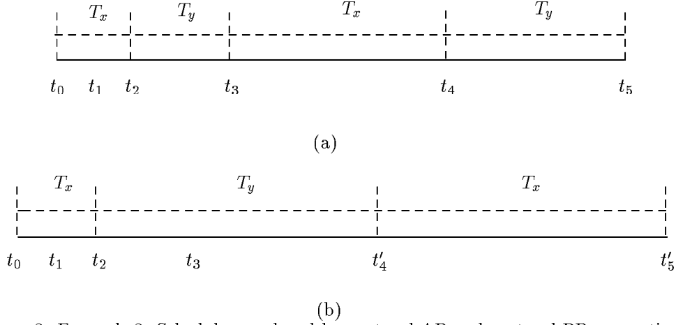
Figure 2: Example 2: Schedules produced by protocol AB and protocol PB, respectively.
