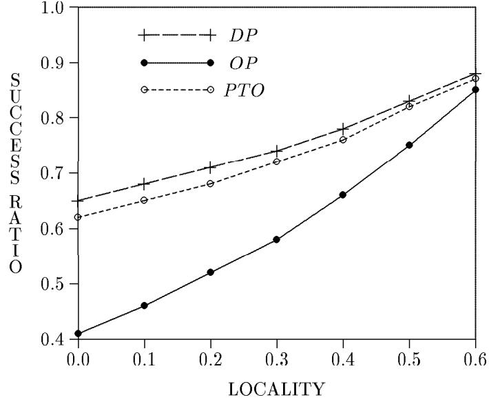
Figure 15: success-ratio vs locality (the probability of referring to a recently accessed data item).
