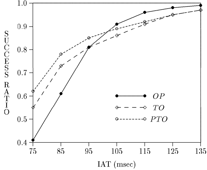
Figure 11: success-ratio vs iat (average transaction interarrival time (msec)) for the timestamp-ordering and optimistic protocols.
