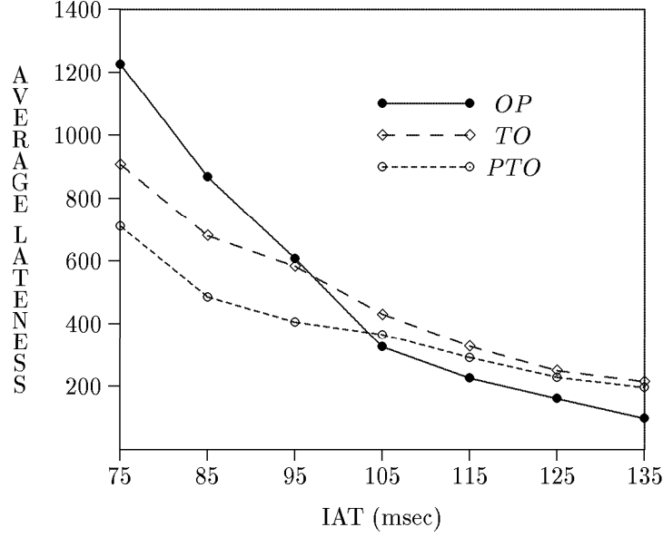
Figure 12: average-latency (msec) vs iat (average transaction interarrival time (msec)) for the timestamp-ordering and optimistic protocols.
