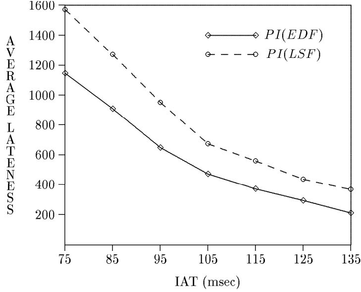
Figure 13: average-latency (msec) vs iat (average transaction interarrival time (msec)) for protocol PI with different priority assignment policies.
