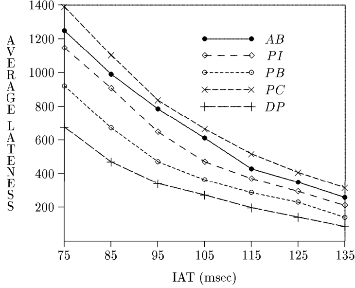
Figure 9: average-latency (msec) vs iat (average transaction interarrival time (msec)) for the locking protocols.
