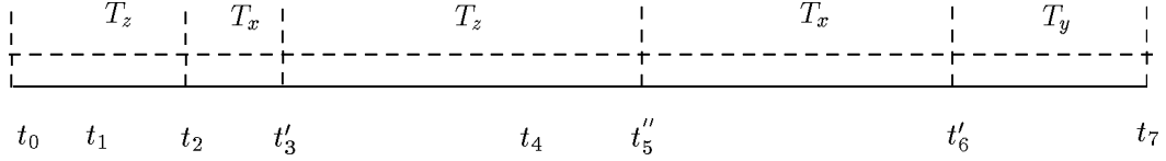
Figure 3: Example 3: Schedule produced by protocol PC.
