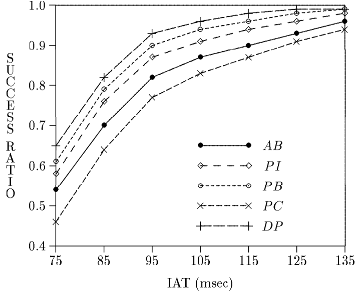
Figure 8: success-ratio vs iat (average transaction interarrival time (msec)) for the locking protocols.
