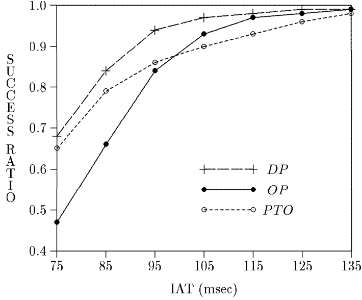
Figure 14: success-ratio vs iat (average transaction interarrival time (msec)) with db-size of 1000 data items and 20/80 data access model.
