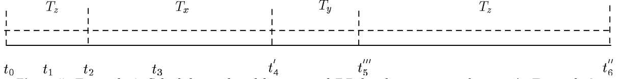
Figure 5: Example 4: Schedule produced by protocol DP for the sequence of events in Example 3.
