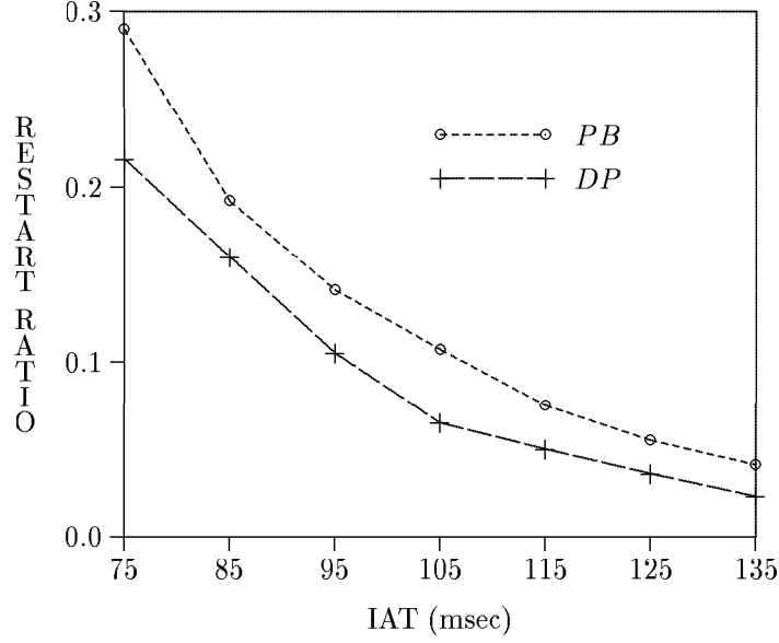
Figure 10: restart-ratio vs iat (average transaction interarrival time (msec)) for protocols PB and DP.
