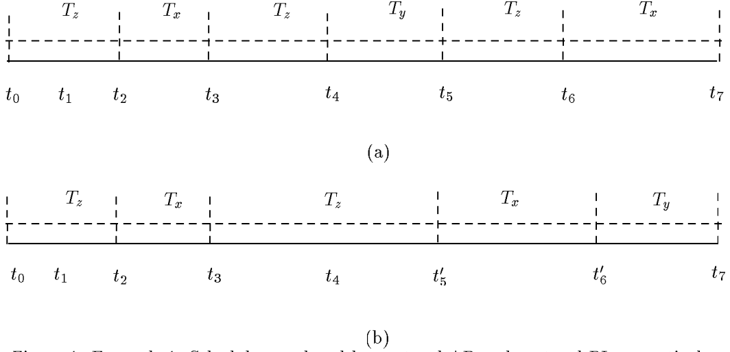
Figure 1: Example 1: Schedules produced by protocol AB and protocol PI, respectively.
