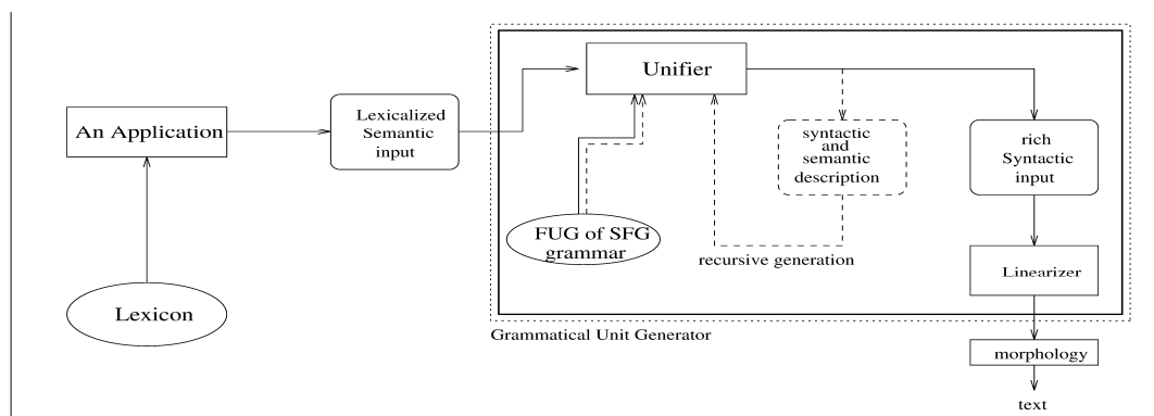
Figure 3: The Architecture of the Text Generator
