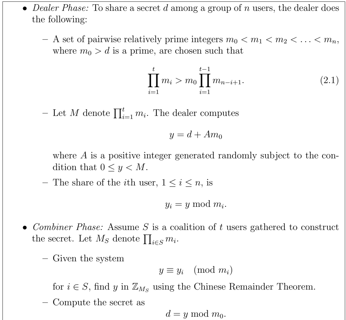
Figure 2.1: The Asmuth-Bloom secret sharing scheme.
