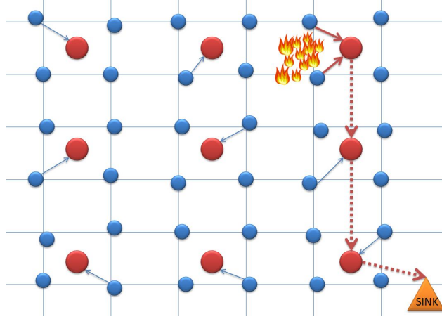
Figure 4.5: Detection of fire event and message forwarding among the nodes
