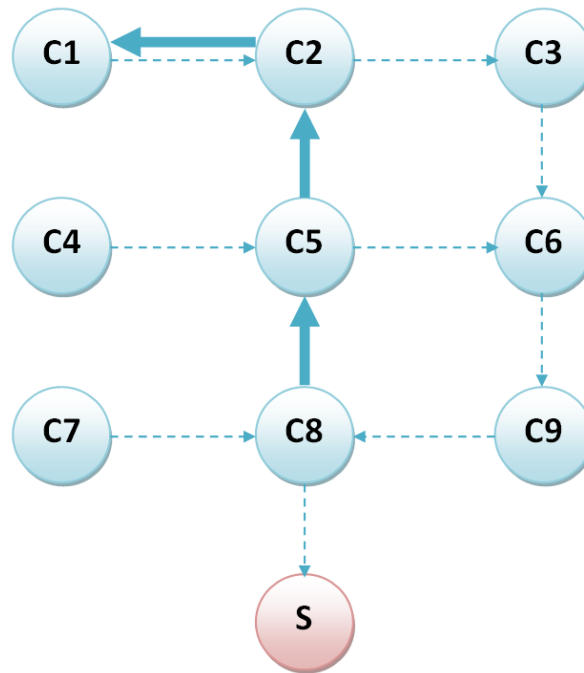
Figure 4.9: Over-hearing scheme at cluster-head level
