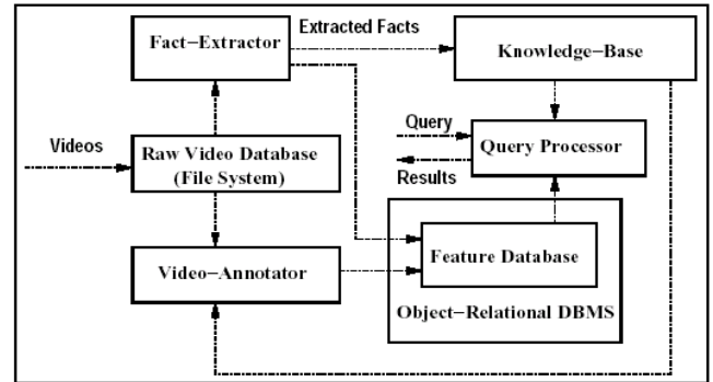
Figure 1: BilVideo System Architecture.
