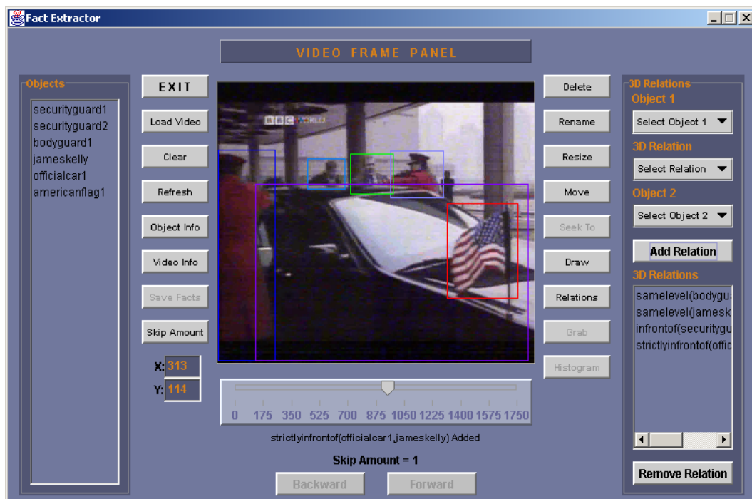
Figure 2: Fact-Extractor
