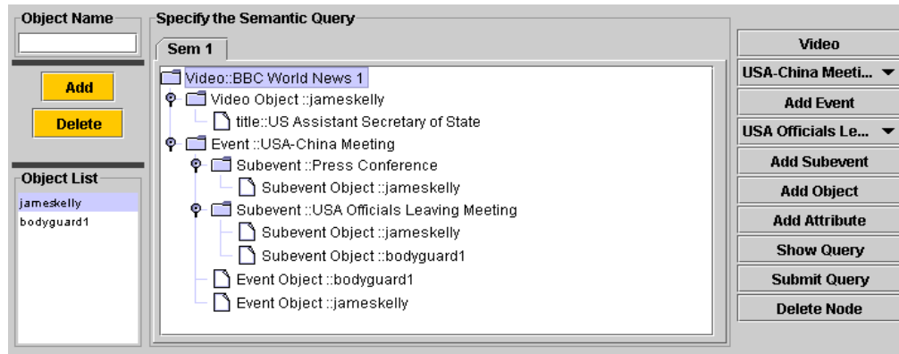
Figure 6: Semantic Query Specification.
