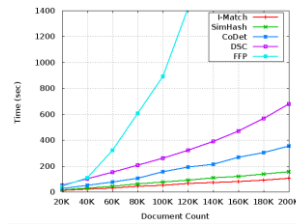
Fig. 3. Efficiency Comparison: Execution Time (sec) vs. Number of Documents.
