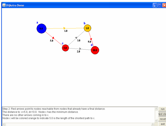
Figure 5. The graph animation module showing the simulation of the Dijkstra's algorithm on a problem specified by the user.
