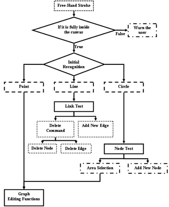
Figure 1. Flowchart for the ink recognition process.
