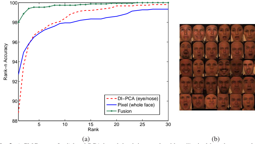
Fig. 3 a) CMC curve for i) local PCA based depth image algorithm, ii) pixel-based texture algorithm and iii) their fusion, and b) Misclassified faces in the v.2 set by the fusion of DI-PCA and TEX-Pixel method.
