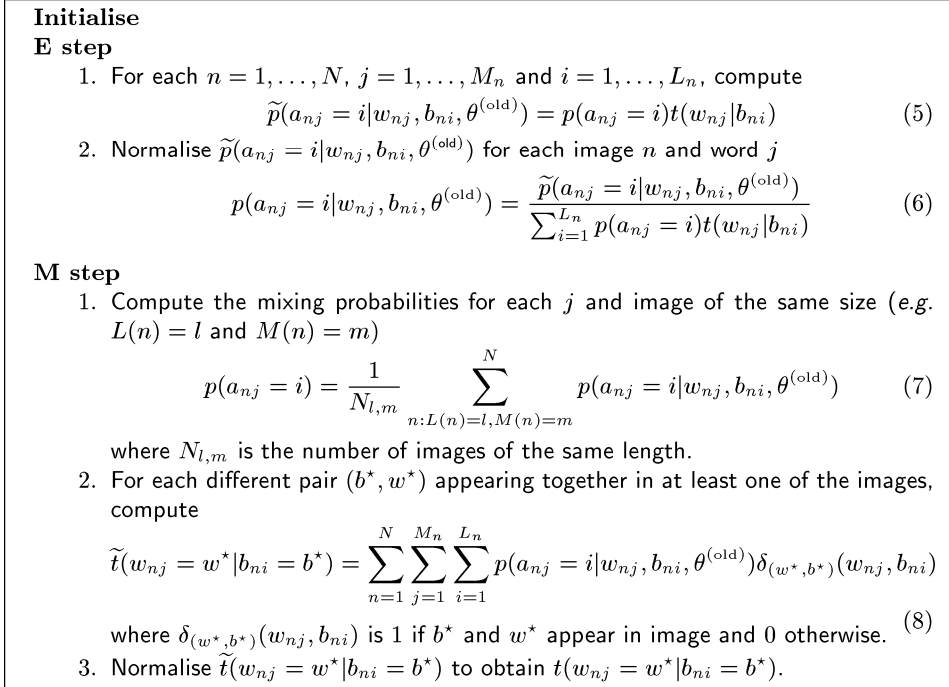
Fig. 4. EM (Expectation Maximization) algorithm
