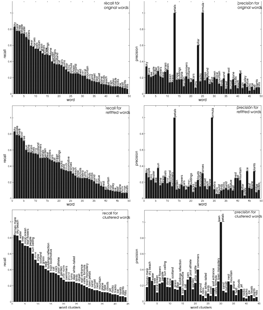
Fig. 5. For 500 test images, left: recall values in sorted order, right: corresponding precision values. top: original words, middle: refitted data, bottom: word clusters. The axes are same in all of the figures. We have some very good words with high recall, and some words with low recall. However, the precision values are not so much different from each other. Although they don't have high recall values, some words have very high precision values, which means that they are not predicted frequently, but when we do predict them we can predict them correctly. When we restrict ourselves only to the reduced vocabulary and run the EM algorithm again, the number of words that we can predict well doesn't change much, but the values increase slightly. Most of the clusters group indistinguishable words into one word, so clustering slightly increases the recall for some clusters (like horse-mare, coral-ocean)
