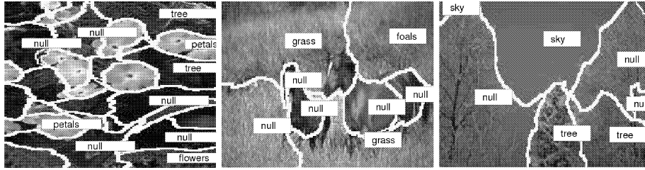
Fig. 10. Result of assigning null. Some low probability words are assigned to null, but the high probability words remain same. This increases the correct prediction rate for the good words, however we may still have wrong predictions as in the last figure. The confusion between grass and foals in the second figure is an example of correspondence problem. Since foals almost always occur with grass in the data, if there is nothing to tell the difference we cannot know which is which.
