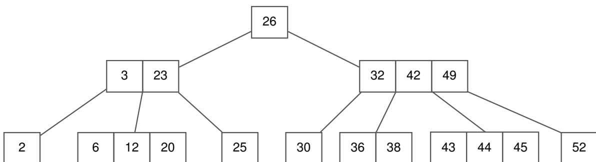
Figure 1: 2-3-4 tree
