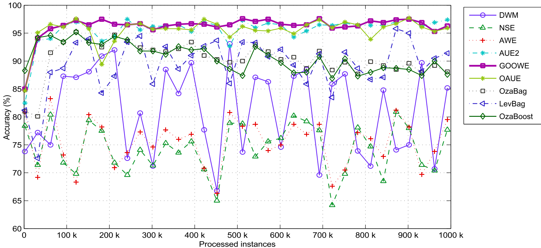
(a) accuracy
