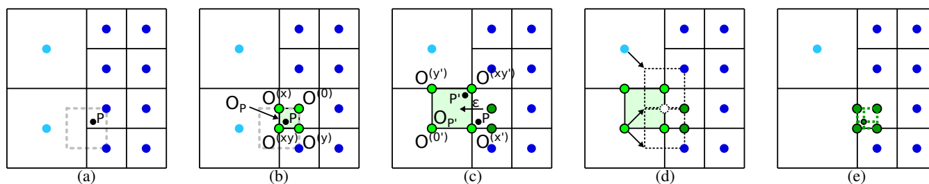
Figure 5: Octant method by Wang et al. [WWW*19]. The octant method presents a rectilinear AMR interpolator that supports smooth reconstruction at level boundaries (a). Interpolation inside an octant (b) defined by corner points O^{(\cdot)} is similar to interpolation using dual cells (dashed rectangle in (a,b)); the corner values can be directly derived from the dual corners. (c) not all the octant corners directly align with data points; then, the coarsest side in the neighbor recursively provides its value to the finer side. To reach the coarse side, the current evaluation position P is offset by a small value \epsilon (e.g., half the width of the finest cell in the data set) in the direction of the coarser cell. (d) Once inside the coarsest side, different strategies exist for how the octant vertices are interpolated from the surrounding cells. (e) When all data values are available, the value at P can be obtained via trilinear interpolation of the octant corner values.
