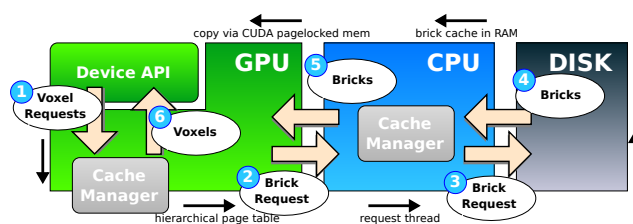
Figure 2: The data path of the framework by Sarton et al. [SCRL20].
