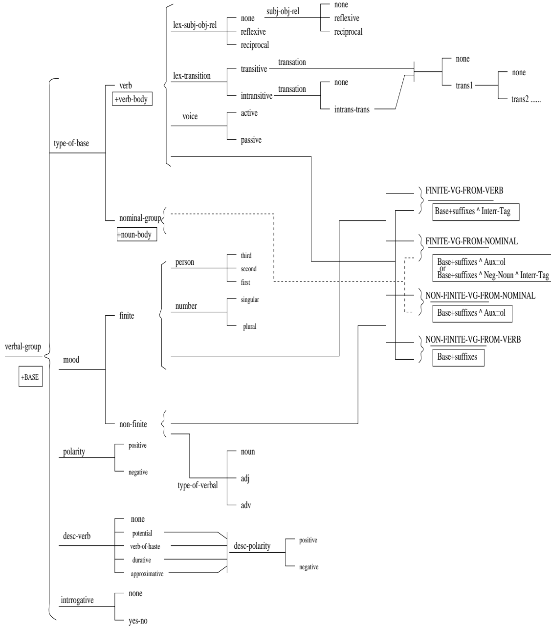
Figure 2: A System Network for Verbal Groups in Turkish
