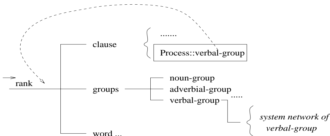
Figure 1: A System Network for the Sentence Generation
