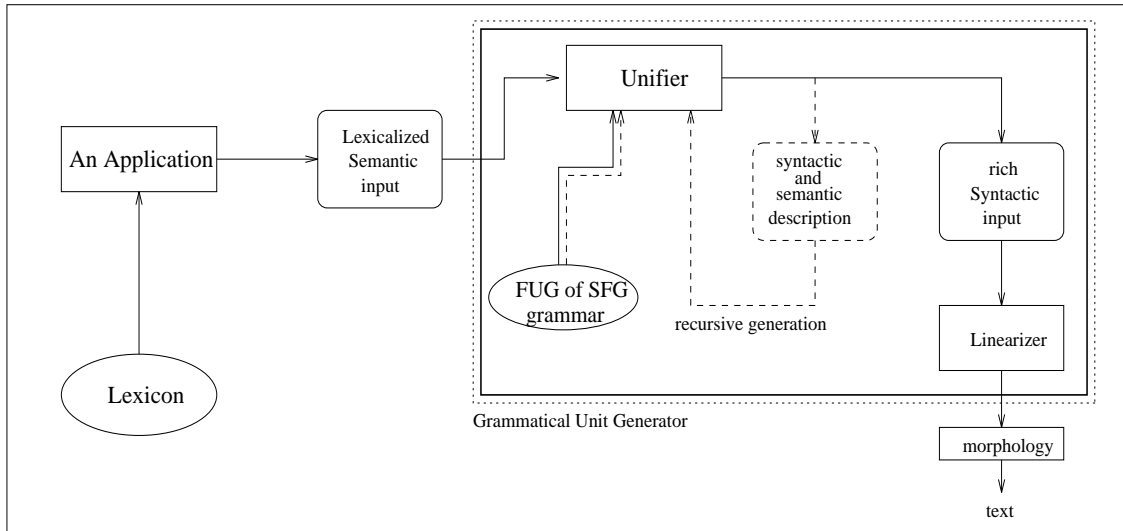
Figure 3: The Architecture of the Text Generator
