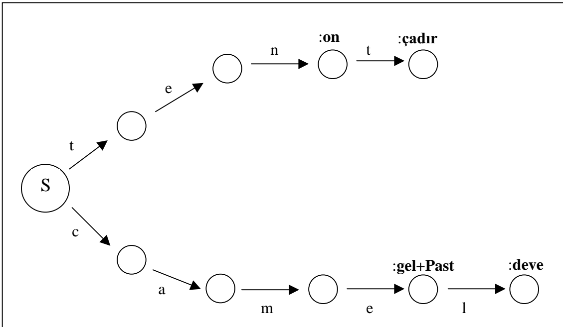
Figure 2. An English-Turkish Dictionary Structure using FST
