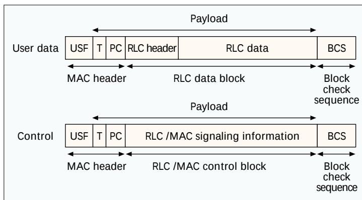
■ Figure 6. GPRS radio block structure.
