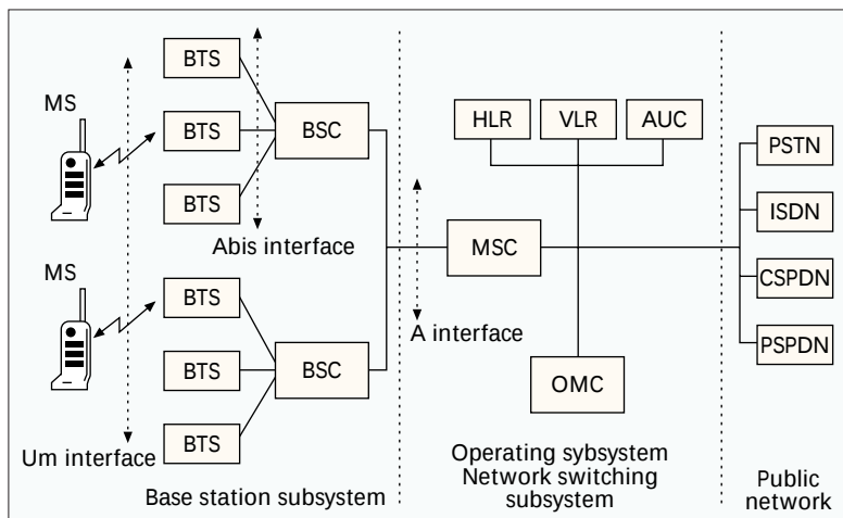
■ Figure 1. GSM system architecture.
