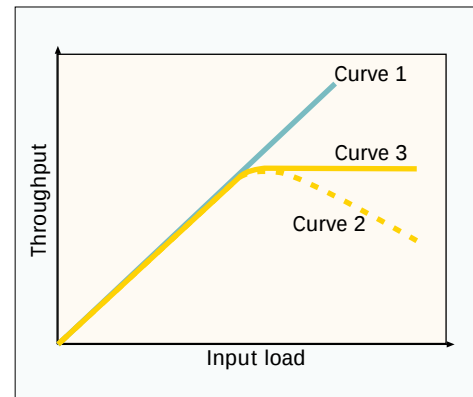
■ Figure 12. Throughput vs. input load in a multi-access system.
