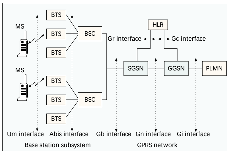
■ Figure 3. GPRS system architecture.
