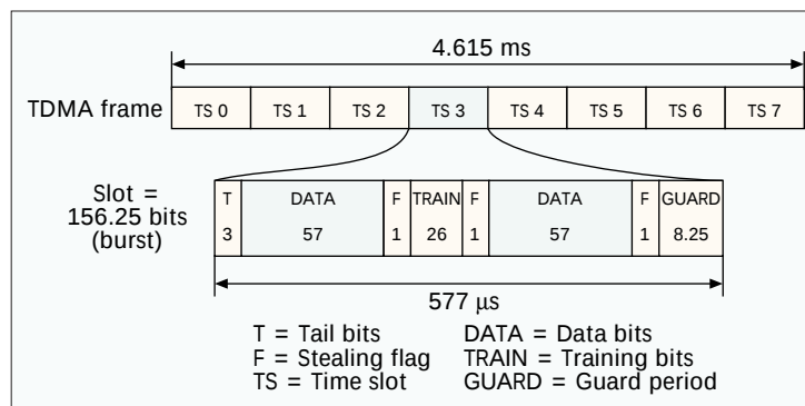
■ Figure 2. GSM burst structure.
