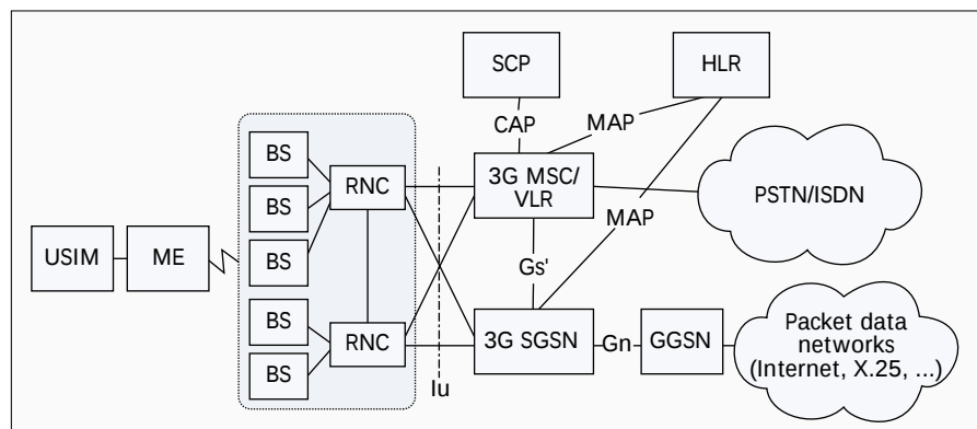
■ Figure 3. One possible scenario where URAN is connected to an evolutionary GSM core network; 3G MSC/VLR and 3G SGSN provide Iu interface.
