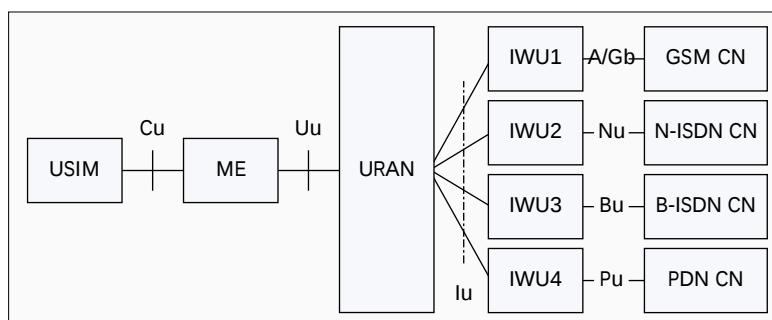
■ Figure 2. General UMTS architecture (figure adapted from [14]).
