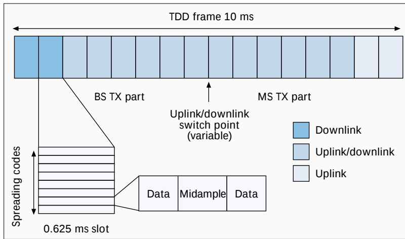
■ Figure 4. An example TDD frame structure.
