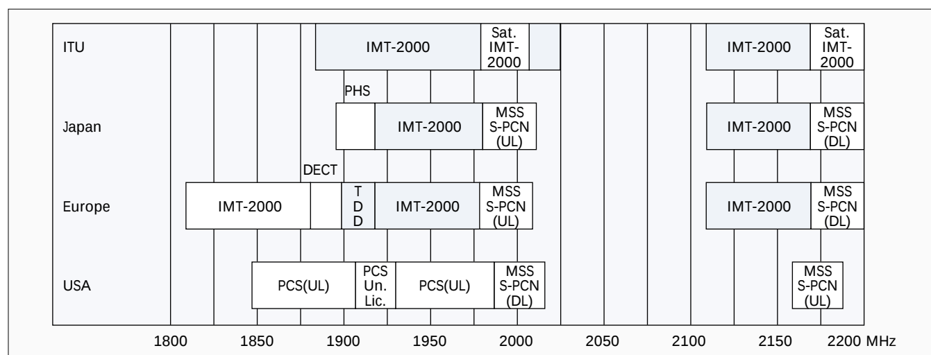
■ Figure 1. IMT-2000 frequency allocations.
