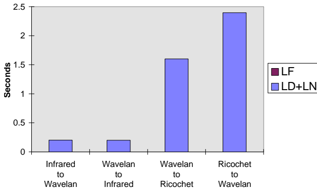
Figure 12. Breakdown of Handoff Latency for the Packet Doublecasting System
