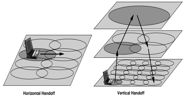
Figure 2. Horizontal vs. Vertical Handoffs
