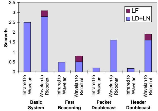
Figure 14. Comparison of Handoff Latency for Basic System and Enhancements
