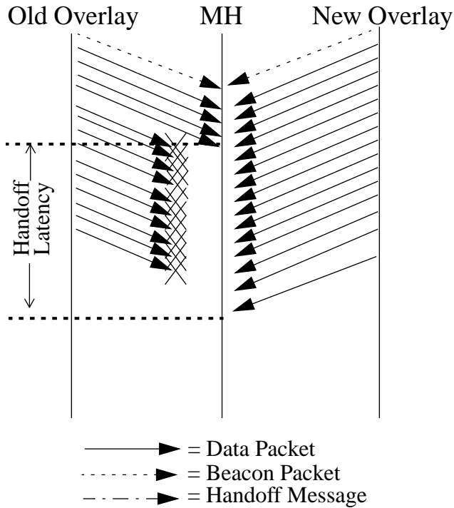
Figure 9. Breakdown of Packet Doublecasting Handoff
