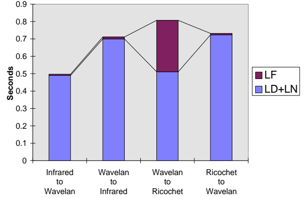
Figure 11. Breakdown of Handoff Latency for the Fast Beaconing System
