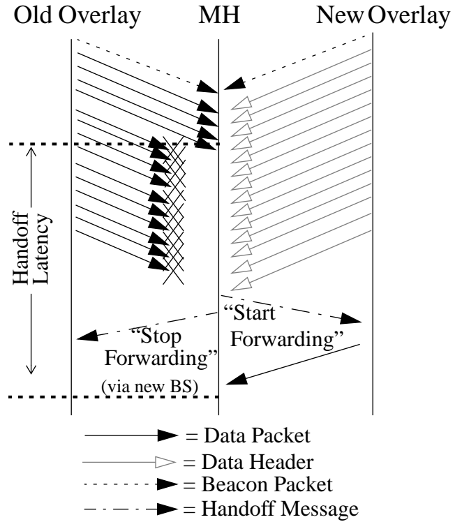
Figure 10. Breakdown of Header Doublecasting
