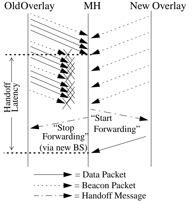
Figure 8. Breakdown of Fast Beacons Handoff
