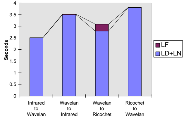
Figure 7. Breakdown of Handoff Latency in Basic System
