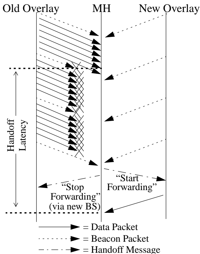
Figure 6. Breakdown of Basic Upward Vertical Handoff
