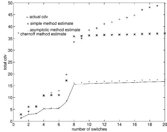
Figure 9: Comparison of estimates and actual end-to-end CDV. Distributions are exponential (special case of Erlang with r = 1 ) with random \lambda values in successive switches.
