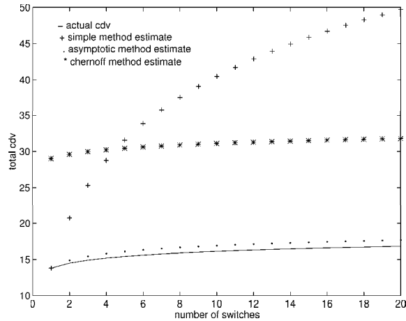
Figure 10: Comparison of estimates and actual end-to-end CDV. Distributions are exponential with increasing \lambda values in successive switches.
