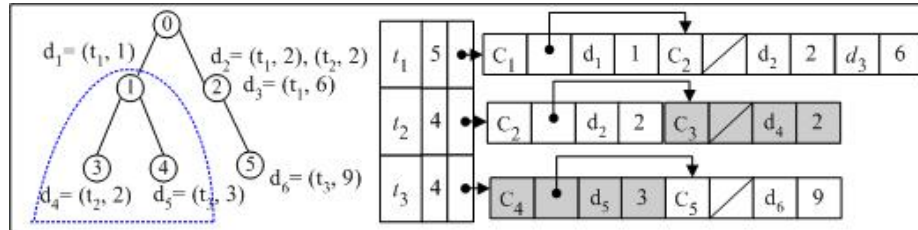
Fig. 1. A hierarchical taxonomy and the corresponding CS-IIS. Given the query = \{t_2, t_3\} that is restricted to C_1 , the query processor first identifies the target categories ( C_1, C_3 and C_4 , as shown within dotted lines) and then processes posting lists. Note that, only the shaded parts of the posting lists are processed and the rest is skipped.
