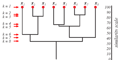
Figure 13: A dendrogram can represent the results of hierarchical clustering algorithms.
