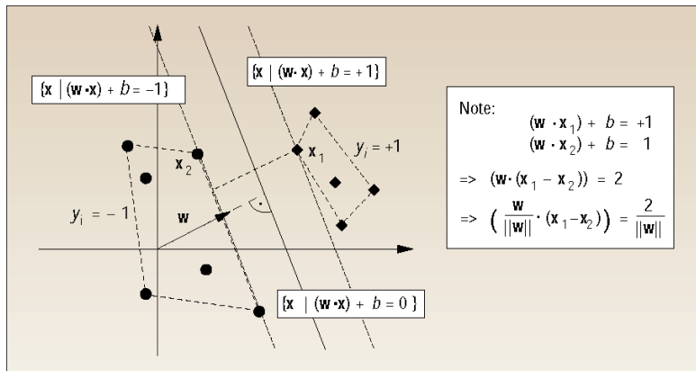
Figure 10: A binary classification problem of separating balls from diamonds. Support vector machines find hyperplane decision boundaries that yield the maximum margin of separation between the classes. The optimal hyperplane is orthogonal to the shortest line connecting the convex hulls of the two classes (dotted), and intersects it half way between the two classes.
