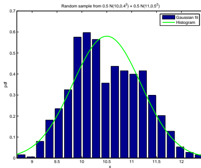
Figure 5: Gaussian density estimation examples.
