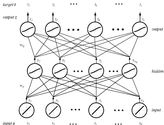
Figure 11: A neural network consists of an input layer , an output layer and usually one or more hidden layers that are interconnected by modifiable weights represented by links between layers. They learn the values of these weights as a mapping from the input to the output.
