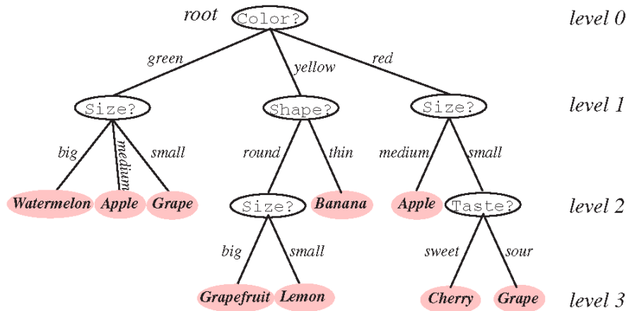
Figure 12: Decision trees classify a pattern through a sequence of questions, in which the next question asked depends on the answer to the current question.
