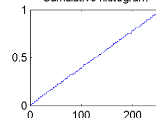
Cumulative histogram
