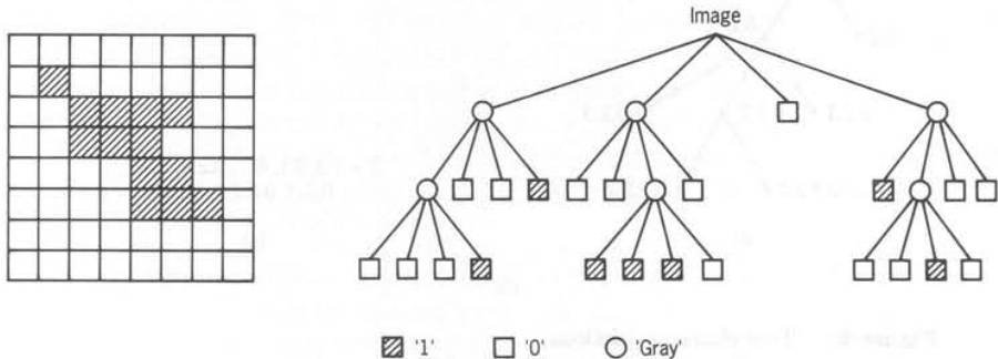
Figure 12: Quadtree representation of an 8 \times 8 binary image.
