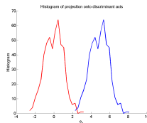
Figure 7: Scatter plot and the PCA and LDA axes for a bivariate sample with two classes. Histogram of the projection onto the first LDA axis shows better separation than the projection onto the first PCA axis.
