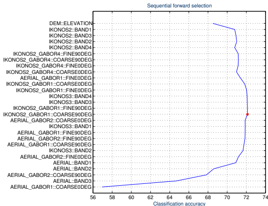
Figure 15: Results of sequential forward feature selection for classification of a satellite image using 28 features. x -axis shows the classification accuracy (%) and y -axis shows the features added at each iteration (the first iteration is at the bottom). The highest accuracy value is shown with a star.
