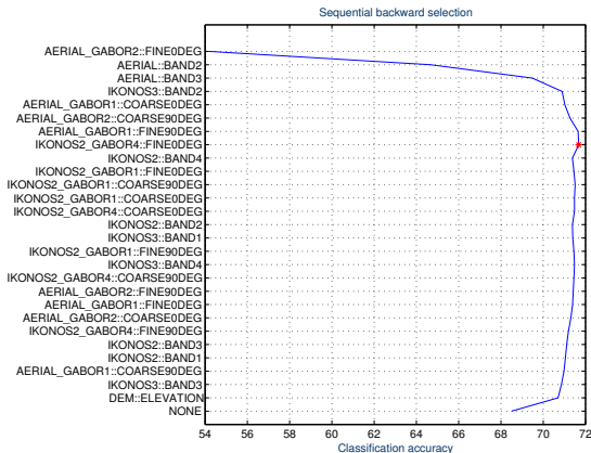
Figure 16: Results of sequential backward feature selection for classification of a satellite image using 28 features. x -axis shows the classification accuracy (%) and y -axis shows the features removed at each iteration (the first iteration is at the bottom). The highest accuracy value is shown with a star.
