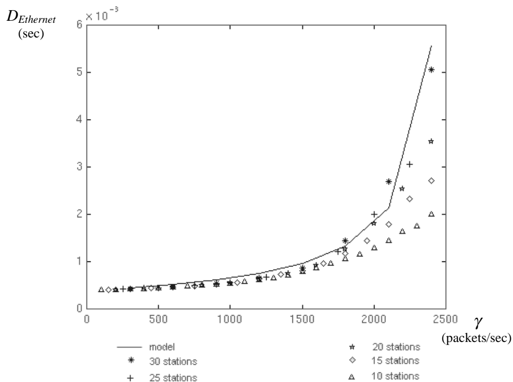
Figure 3. Accuracy of the Ethernet analytical model.
