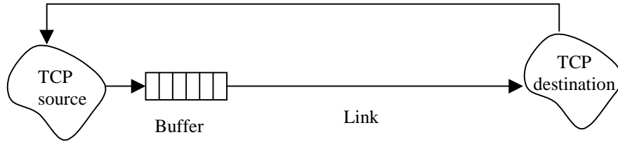
Figure 1. Simple data transmission model.
