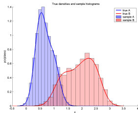
(a) True densities and sample histograms.
