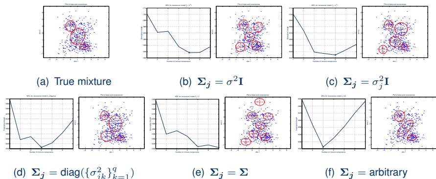
Figure 6: Example fits for a sample from a mixture of three bivariate Gaussians. For each covariance model, description length vs. the number of components (left) and fitted Gaussians as ellipses at one standard deviations (right) are shown. Using MDL with the arbitrary covariance matrix gave the smallest description length and also could capture the true number of components.
