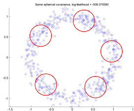
(b) Same spherical covari- ance, log-likelihood = -806.08.
