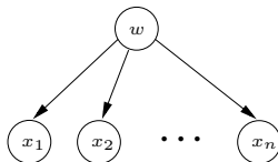
Figure 12: Naive Bayesian network structure. It looks like a very simple model but it often works quite well in practice.
