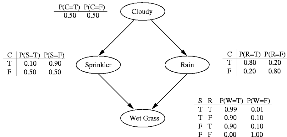
Figure 11: Another Bayesian network example. The event that the grass being wet ( W = \text{true} ) has two possible causes: either the water sprinkler was on ( S = \text{true} ) or it rained ( R = \text{true} ). (Russell and Norvig, Artificial Intelligence: A Modern Approach, 1995)
