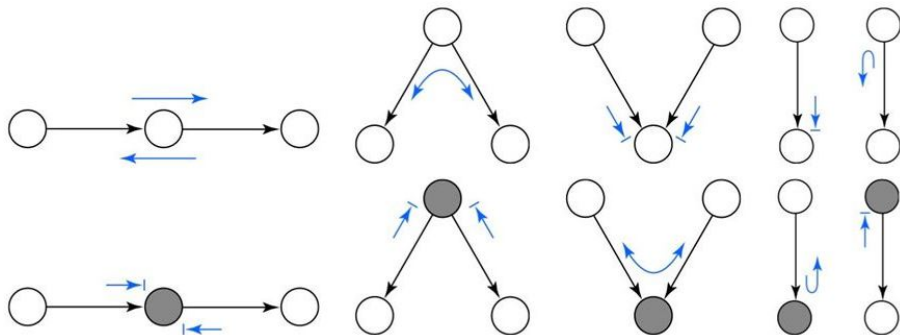
Figure 9: Ten rules of the Bayes ball algorithm. A path is active if a Bayes ball traveling along it never encounters the stop symbol . (Observed nodes are shaded, unobserved nodes are empty.)
