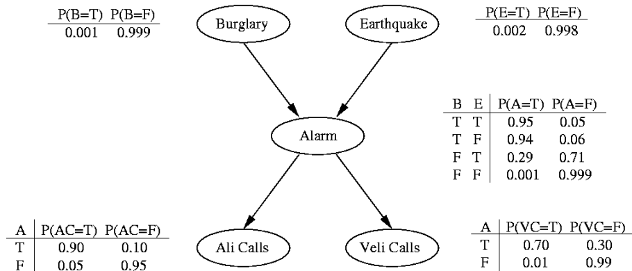
Figure 10: The Bayesian network for the burglar alarm example. Burglary (B) and earthquake (E) directly affect the probability of the alarm (A) going off, but whether or not Ali calls (AC) or Veli calls (VC) depends only on the alarm. (Russell and Norvig, Artificial Intelligence: A Modern Approach, 1995)
