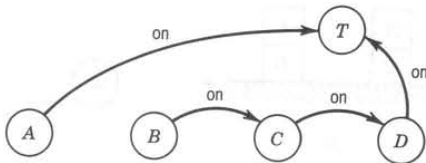
Figure 13: A grammar describing four blocks arranged in 3-block and 1-block stacks. (i) An example. (ii) Graphical description corresponding to (i). (iii) Another example. (iv) Graphical description corresponding to (iii).
