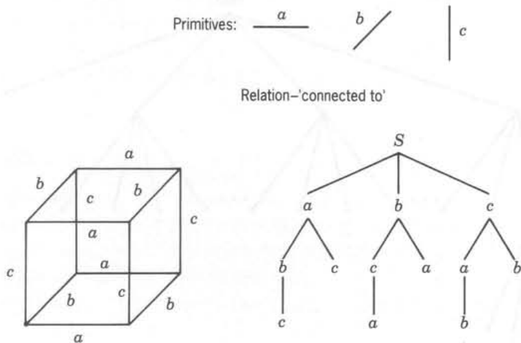
Figure 14: Tree grammar-based representation of a cube.
