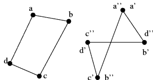
Figure 1: An example of isomorphism of two undirected graphs with p = 4 .
