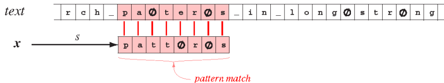
Figure 7: The problem of string matching with the “don’t care” symbol is the same as the basic string matching except that the \emptyset symbol can match any character. The figure shows the only valid shift.
