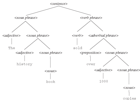
Figure 8: The derivation tree illustrates how a portion of English grammar can transform the root symbol into a particular sentence.
